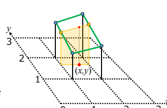
Bilinear Interpolation
