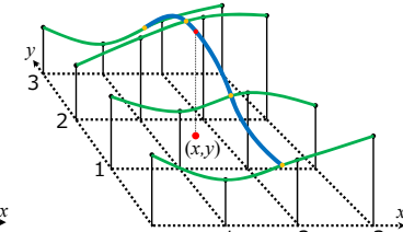
Bicubic Interpolation
