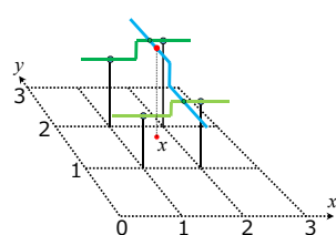
Nearest Neighbor
